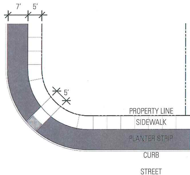
Sidewalk Dimensions
