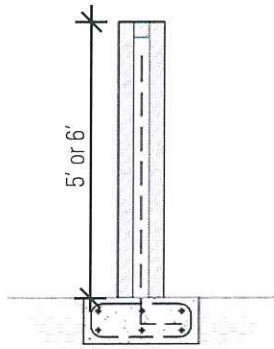
Type 'A' Fence Cross Section
