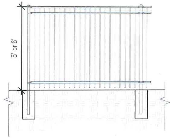
Type 'B' Fence
