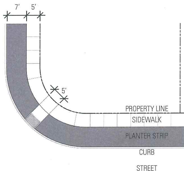
Sidewalk Dimensions
