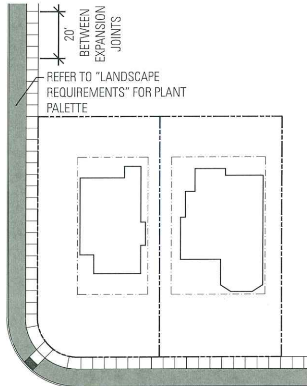
Sidewalk Exhibit
